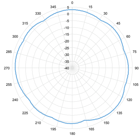
2.4 GHz Elevation
