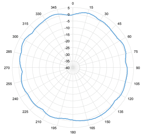
5 GHz Elevation
