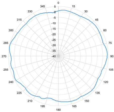
5 GHz Azimuth
