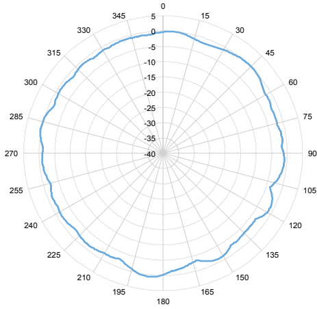
2.4 GHz Azimuth
